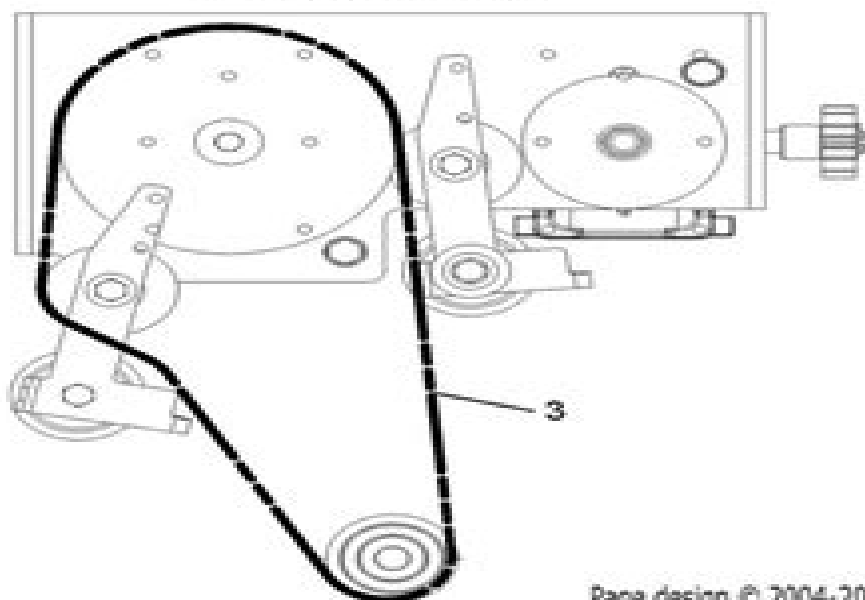
REVERSE BELT ROUTING
