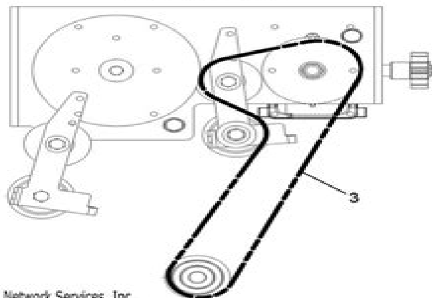
FORWARD BELT ROUTING
