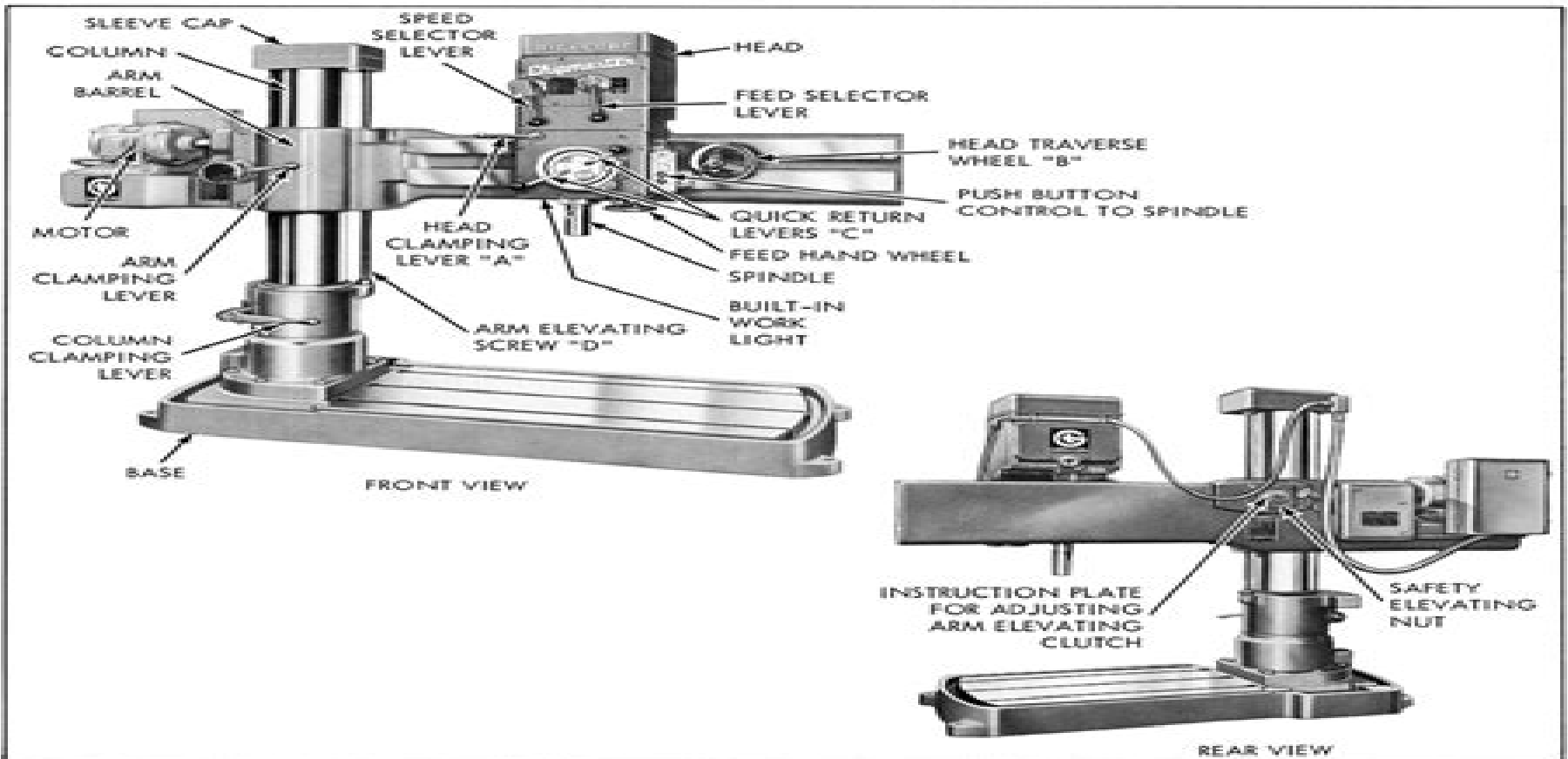
Figure 1-1. Giddings & Lewis Bickford 9-inch Radial Drilling Machine
