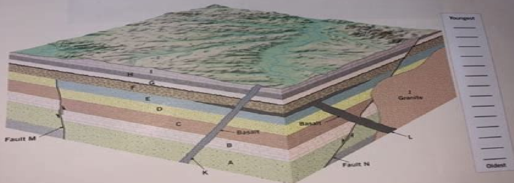
Figure 10.24 Geologic block diagram of a hypothetical region.
