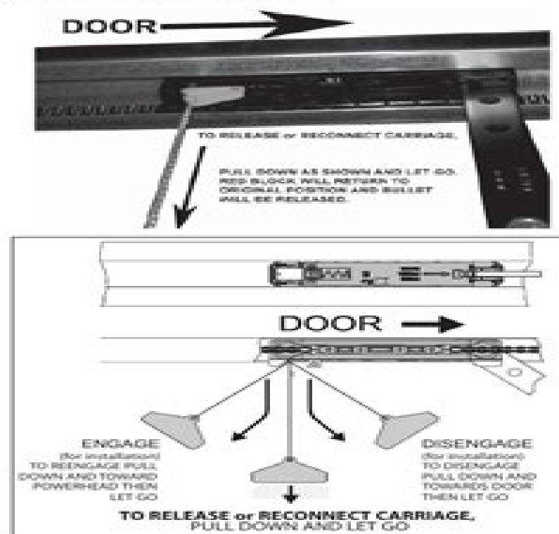
FIG. 6-4 Carriage Release (cut away view) 12/2010
