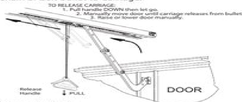
FIG. 6-3 Carriage Release
