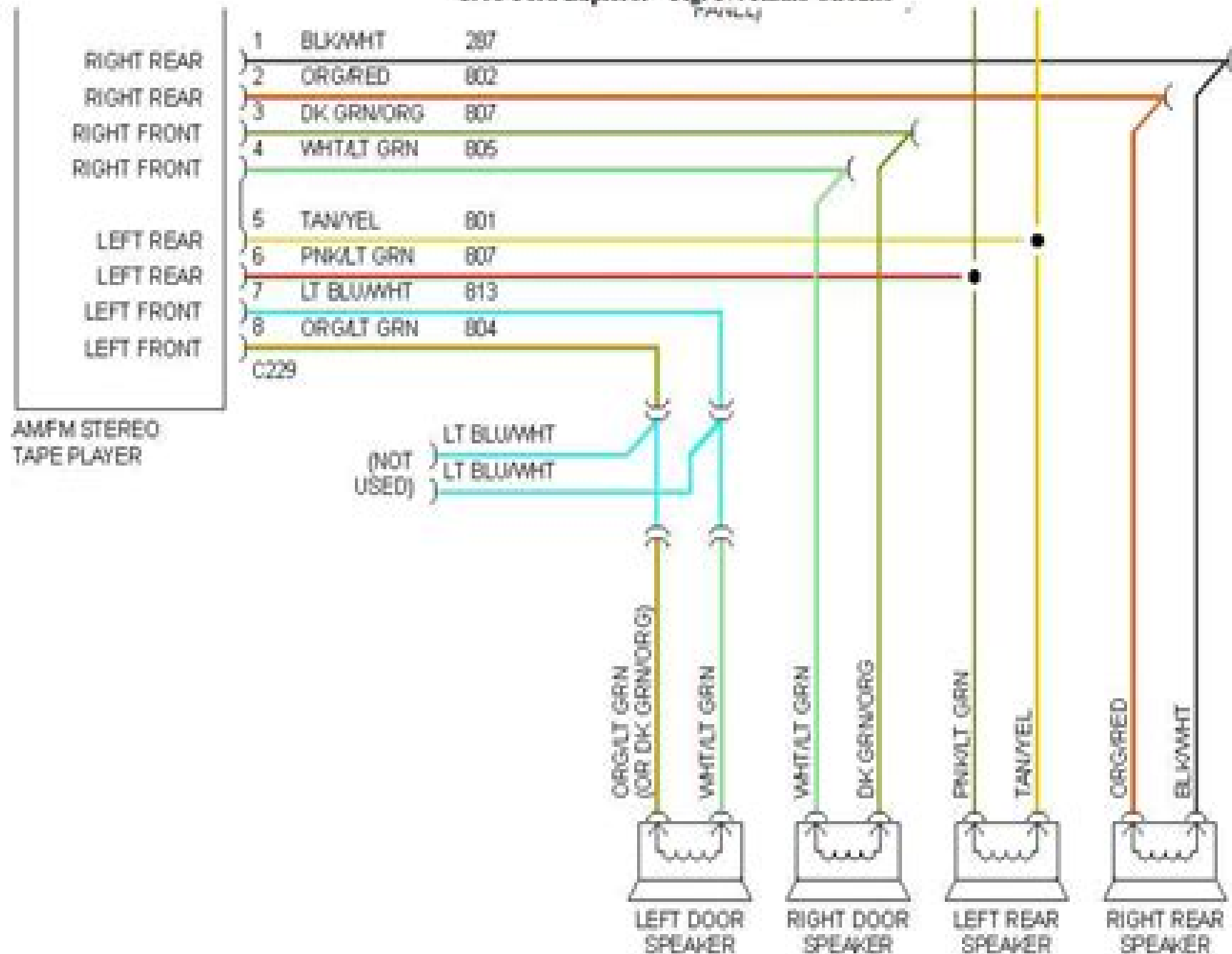
1993 Ford Explorer - Fig. 17: Radio Circuits
