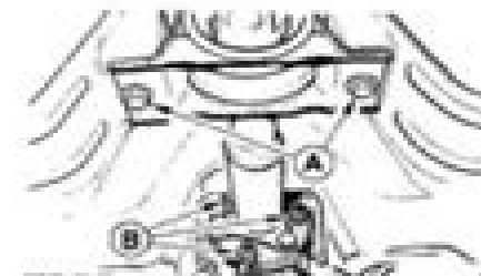
Fig. 20. Fixature of driveshaft. A - Centre bearing balls B - Transmission output flange nuts
