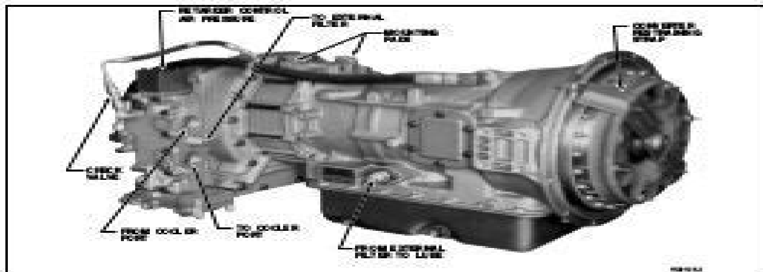
Figure 1-7. Model MTB 65B Automatic Transmission — Right-Front View
