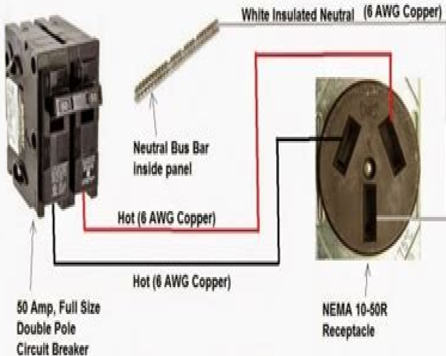
50 Amp, 3 wire Range Circuit
