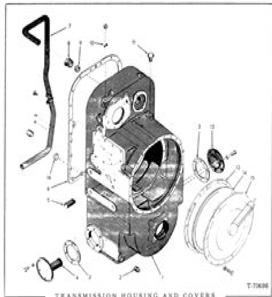
TRANSMISSION HOUSING AND COVERS
