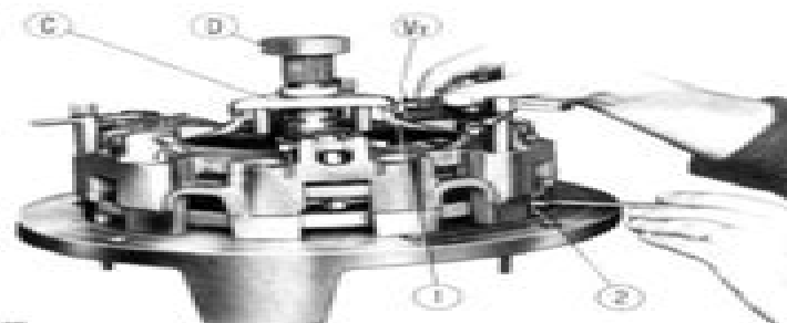
On-Bench Inspection and Adjustment of P.T.O. Clutch Release Lever Height Using Tool 291291/2 or Universal tool 293650
