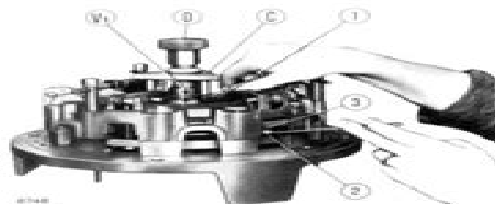
On-Bench Inspection and Adjustment of Transmission Clutch Release Lever Height Using Tool 291291/2 or Universal tool 293650
