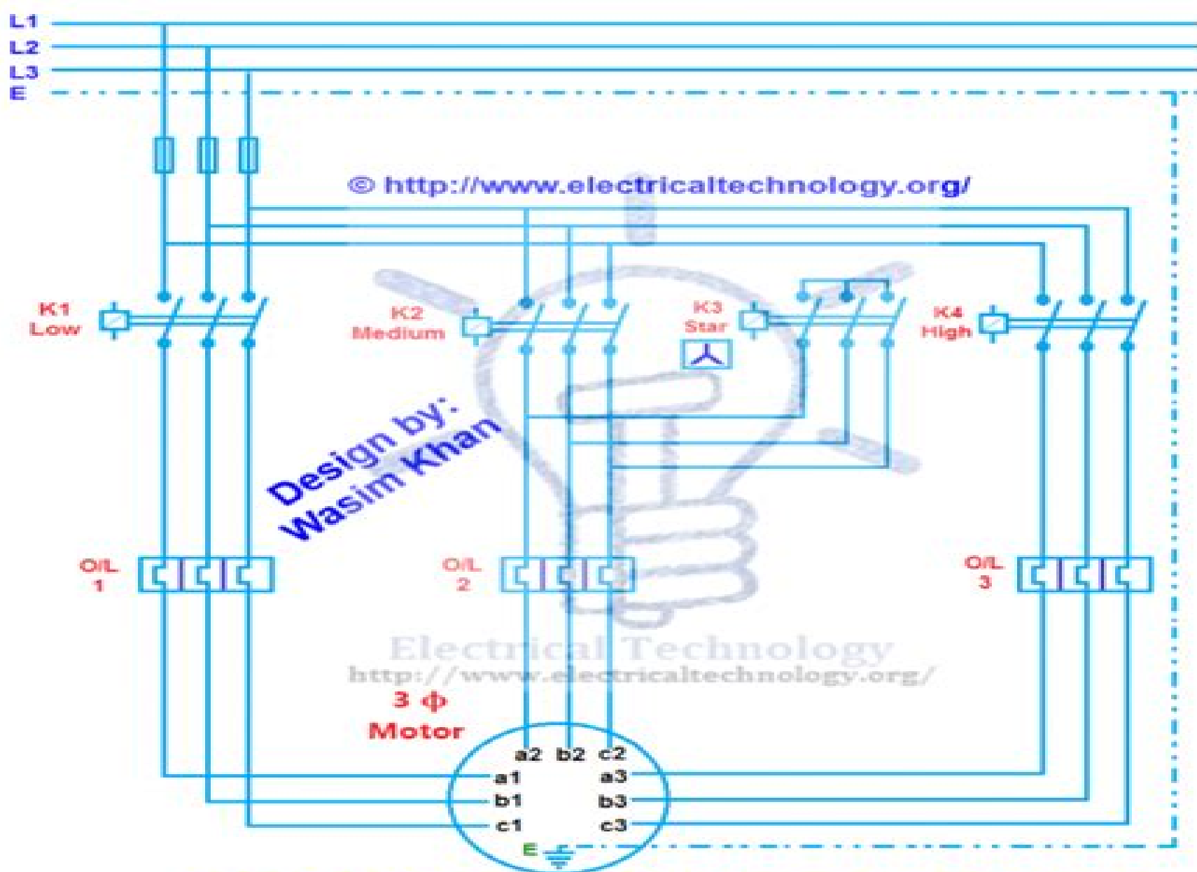
Multi Speed 3-Phase Motor 3 Speed, 1 Direction, Power Diagram
