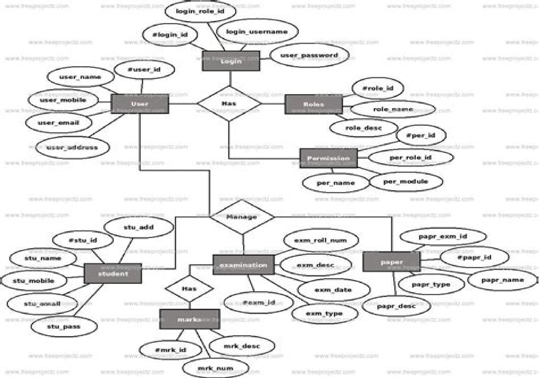
ER Diagram For Examination Management System
