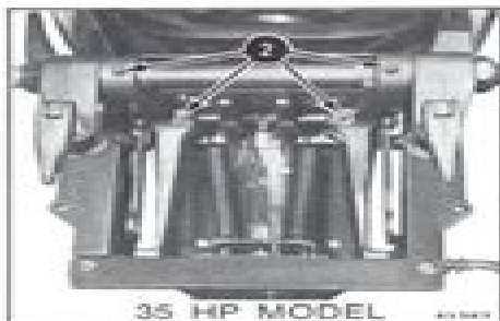
Figure 2-3. Tilt Tube and Tilt Lever Shaft
