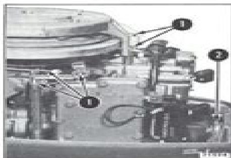
Figure 2-1. Throttle and Shaft Linkage, Rear Motor Cover Latch, Starter Neutral Lockout (Manual Start)
