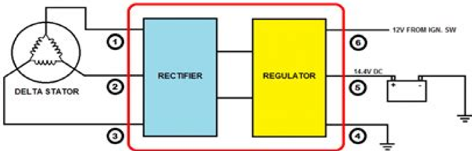
3-PHASE REGULATOR
