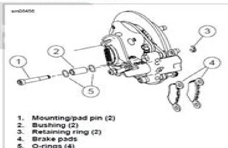
Figure 1-8. Rear Brake Caliper Assembly
