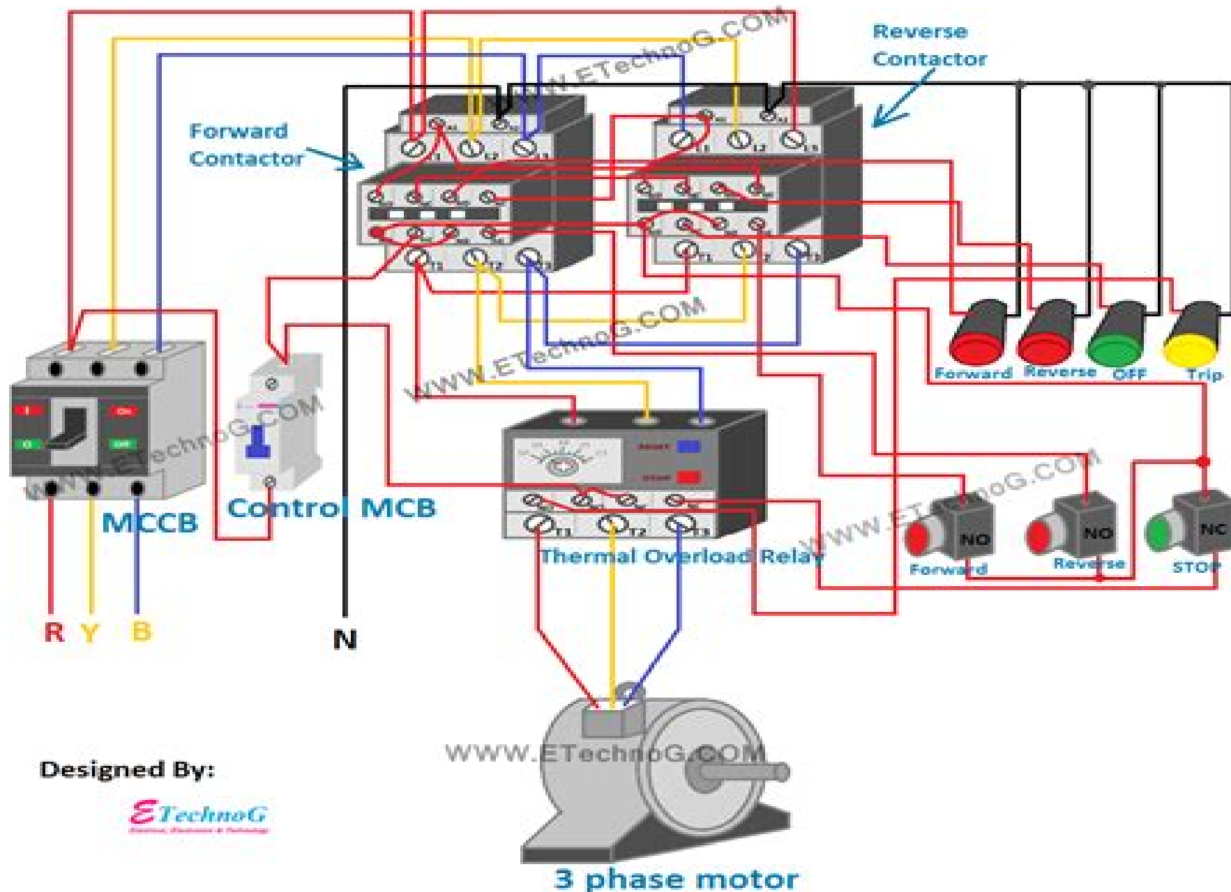
Motor Control Circuit Forward Reverse | Wiring and Connection
