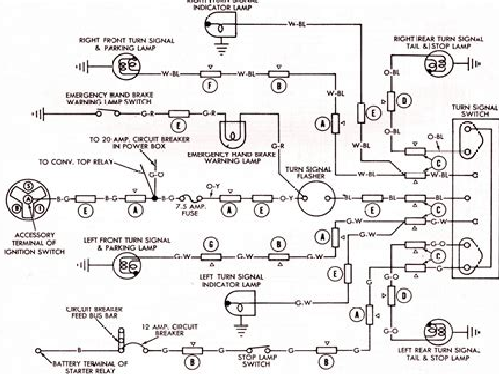
1961-63 Lincoln turn signal circuit.
