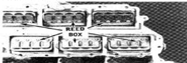
Six reed boxes mounted in the reed plate of a V6 powerhead.
