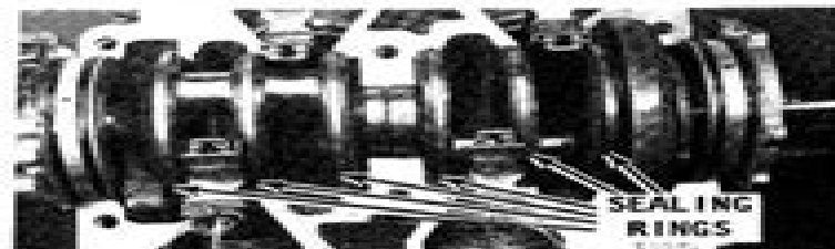
V4 engine block with sealing rings to hold pressure and vacuum within each cylinder.
