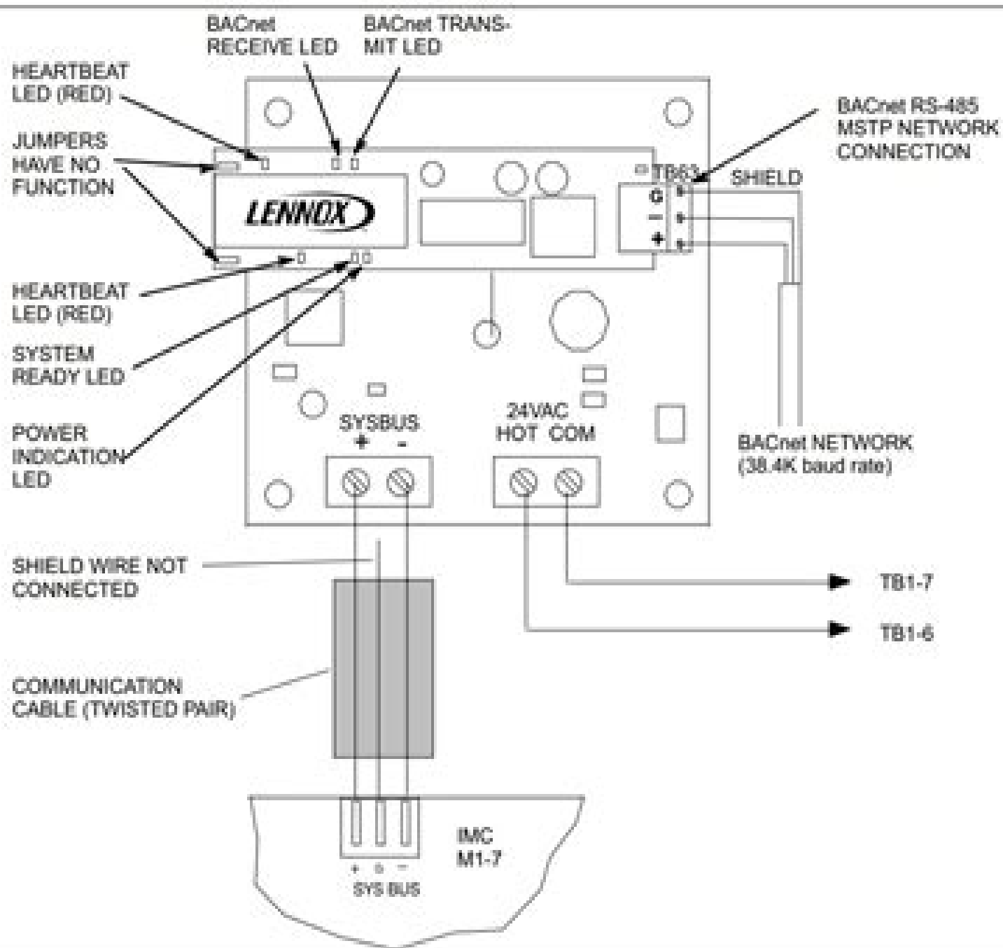
Figure 1. IMC BACnet® Module (A146)
