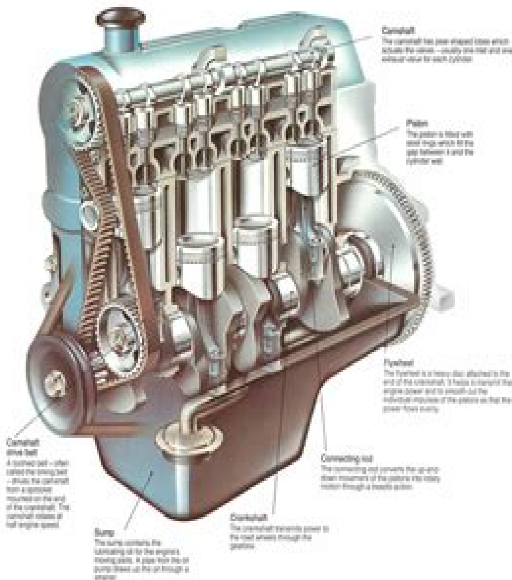
The parts of an overhead-camshaft engine
