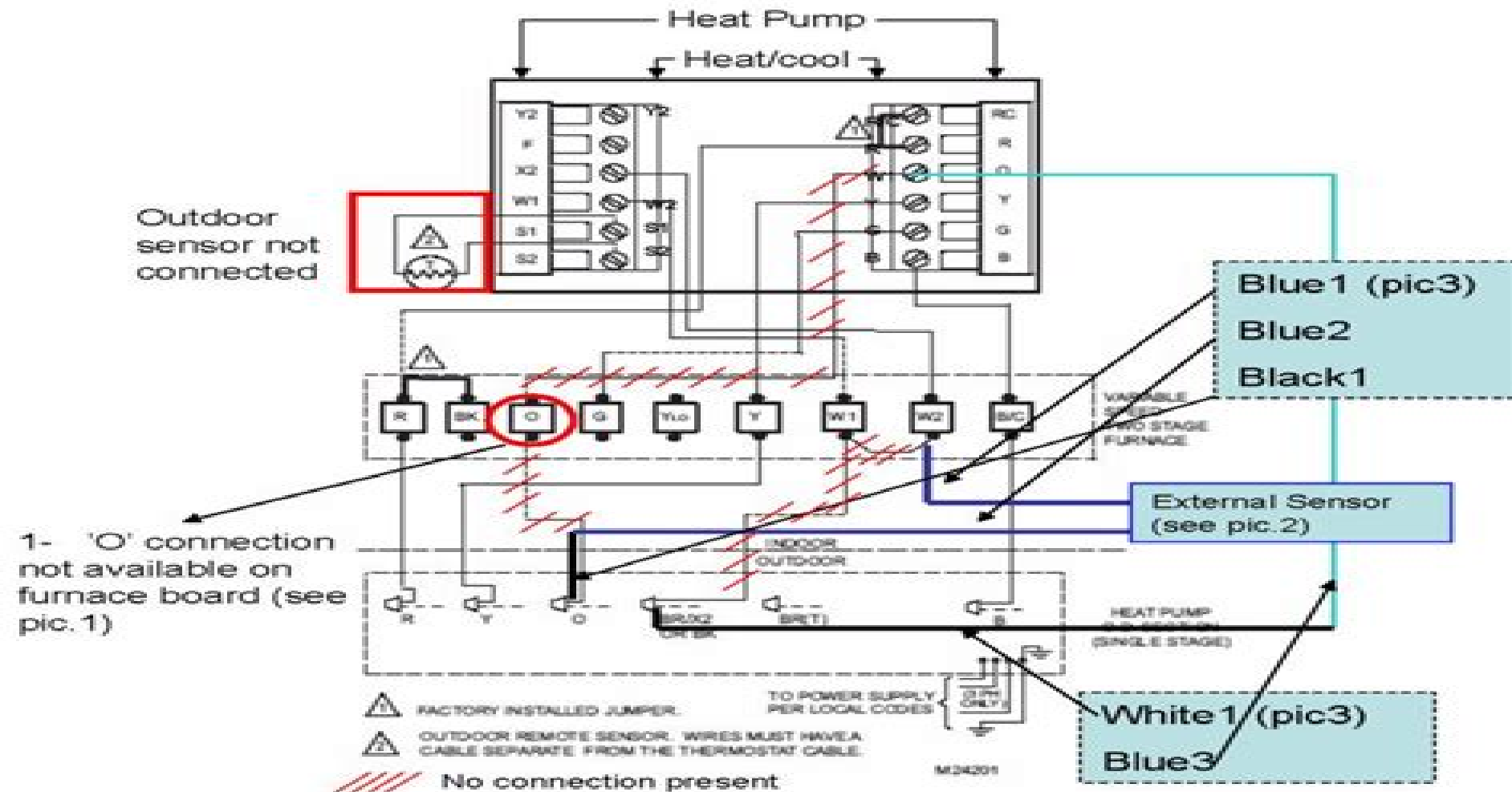
Fig. 13. Typical hookup of single-stage heat pump with two stage variable speed gas furnace (2H/1C heat pump).
