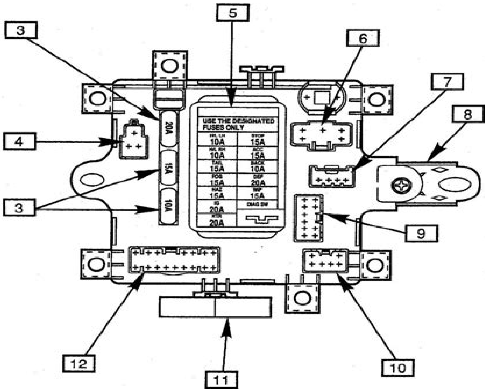
Junction Block, Bottom View
