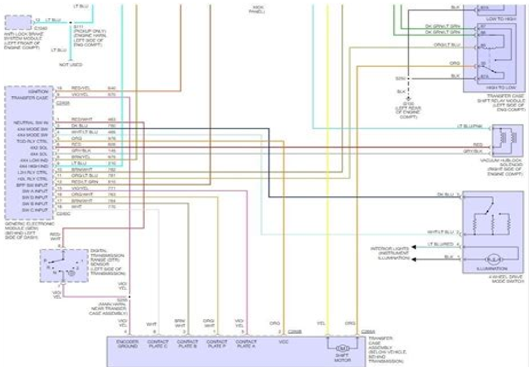
Fig 1: 4WD Circuit
