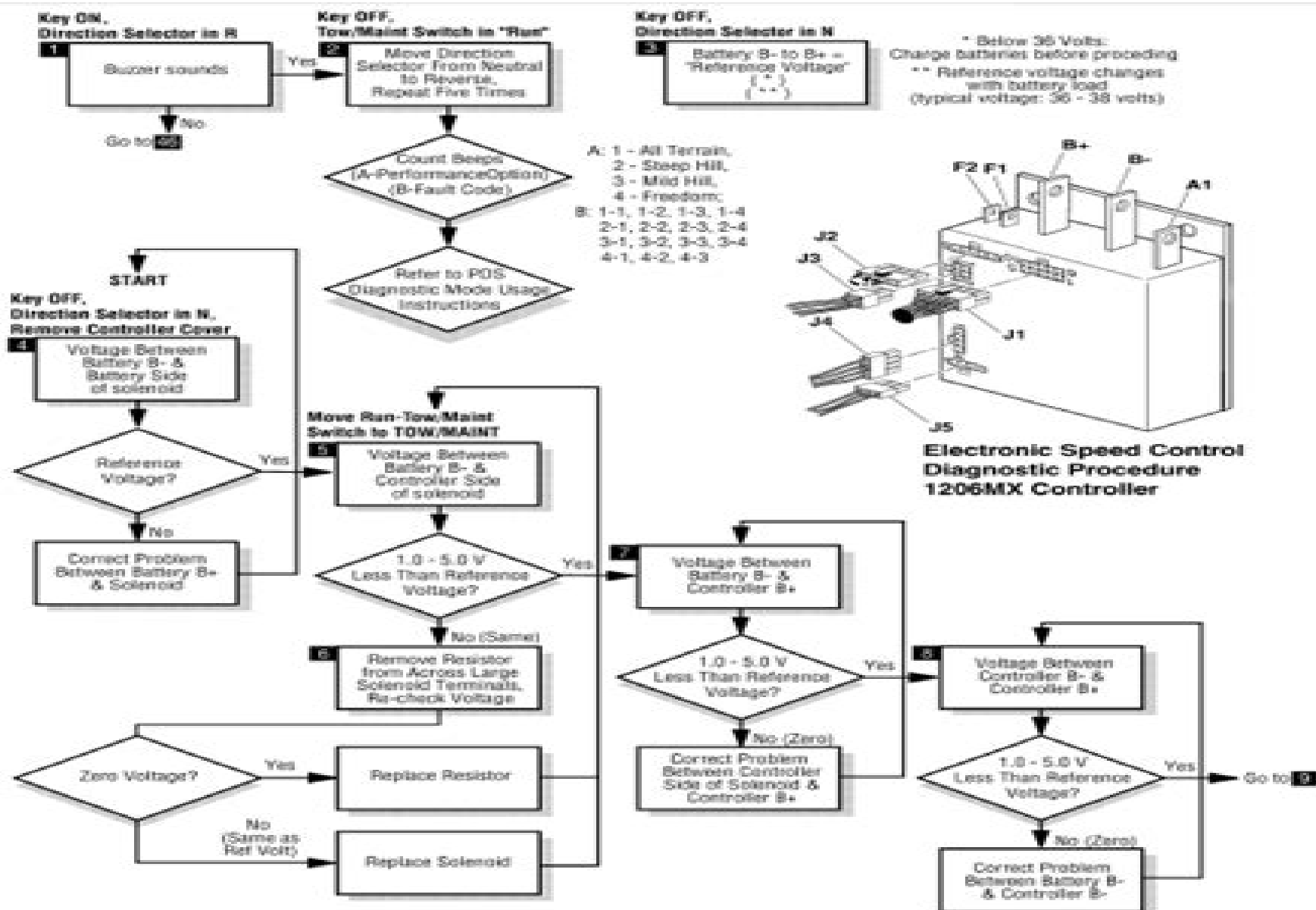
Fig. 10 Detailed Troubleshooting Diagram (Sheet 1 of 10)
