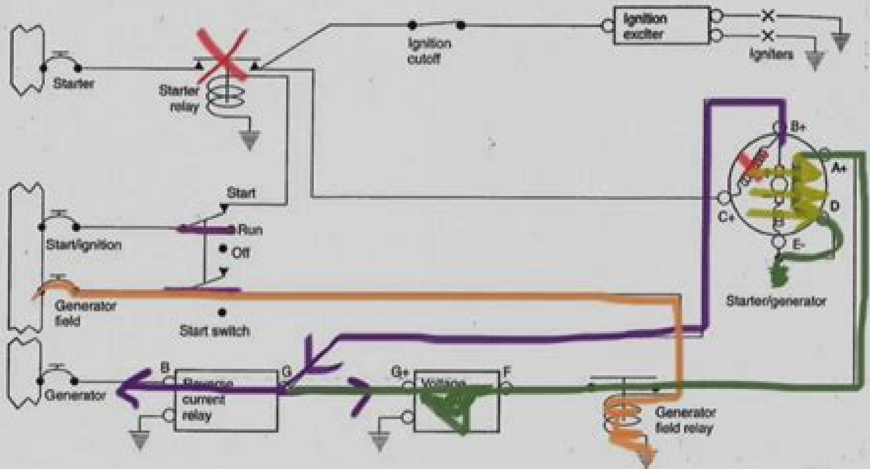
Figure 13-9. Basic starter-generator circuit
