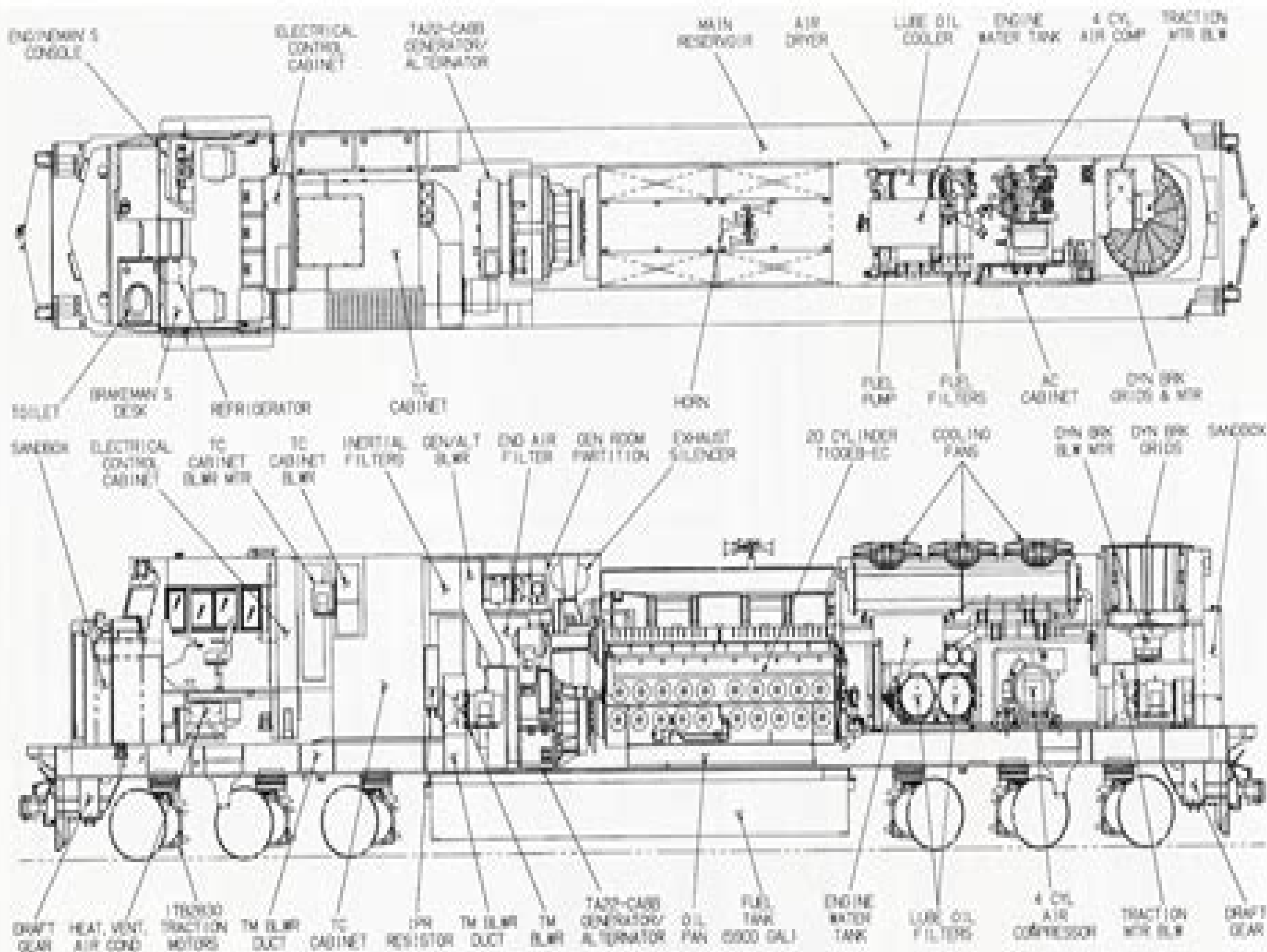
EQUIPMENT LOCATION
