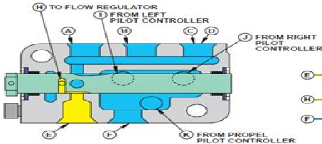
(L) PILOT SHUT-OFF VALVE OFF
