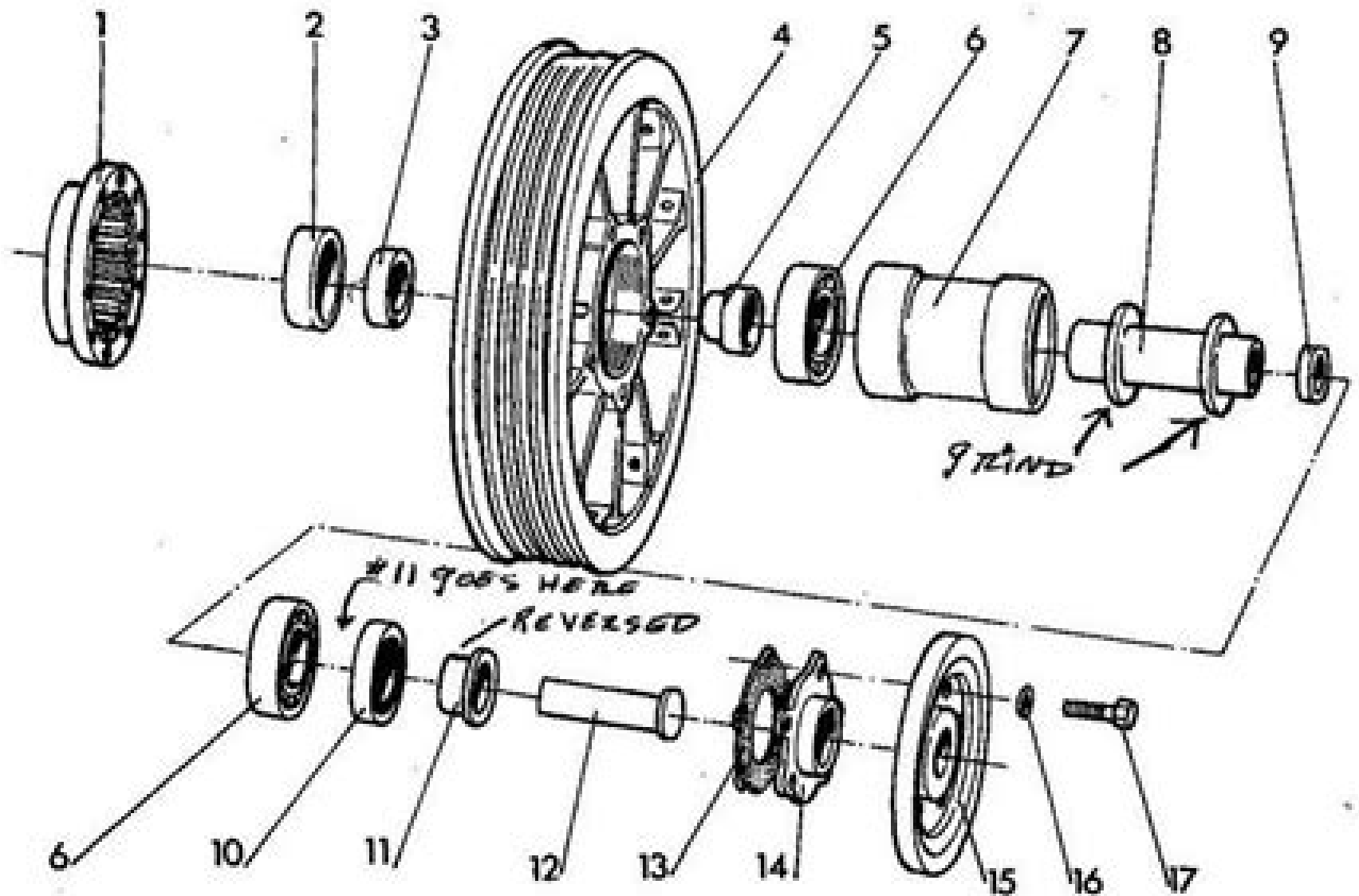
Fig. 7.4. Drum brake wheel hub
