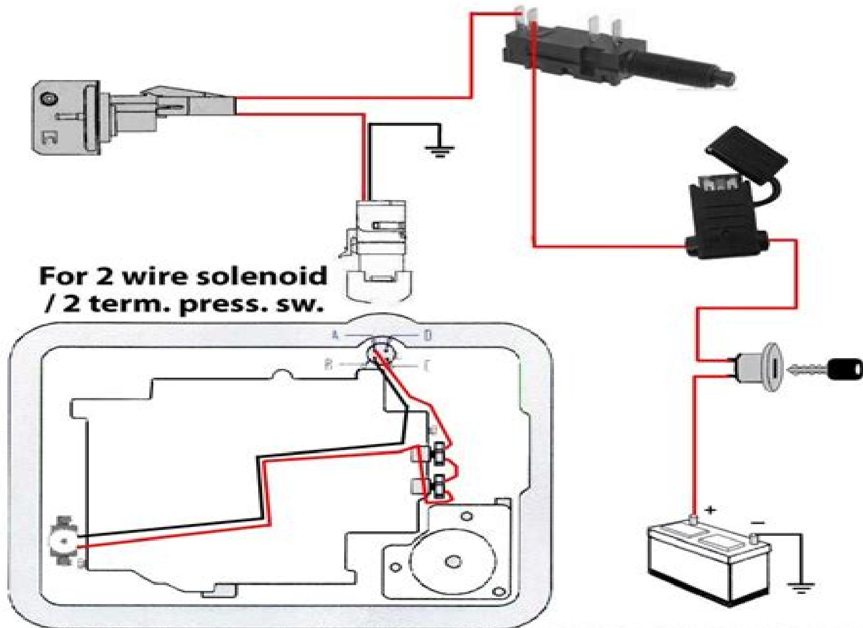
700R4 non-computer TCC wiring
