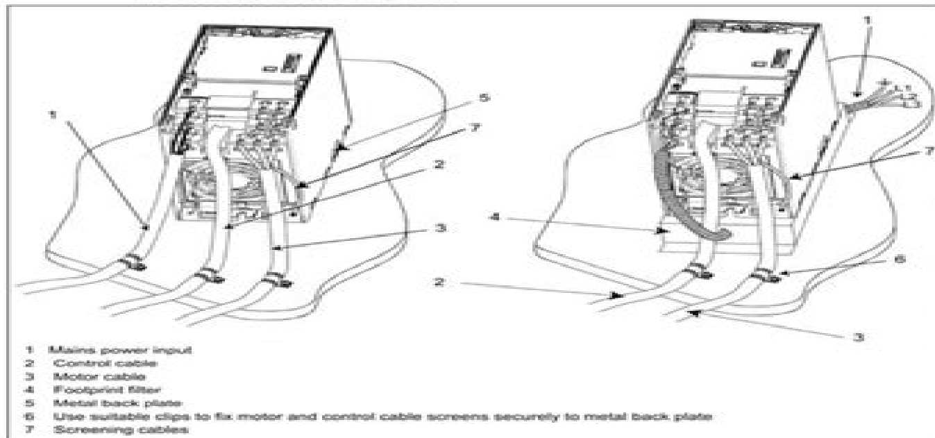
Fig. 2-14 Wiring Guidelines to Minimize the Effects of EMI
