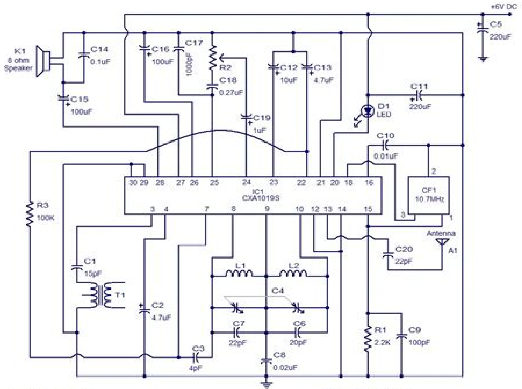
FM Radio receiver circuit
