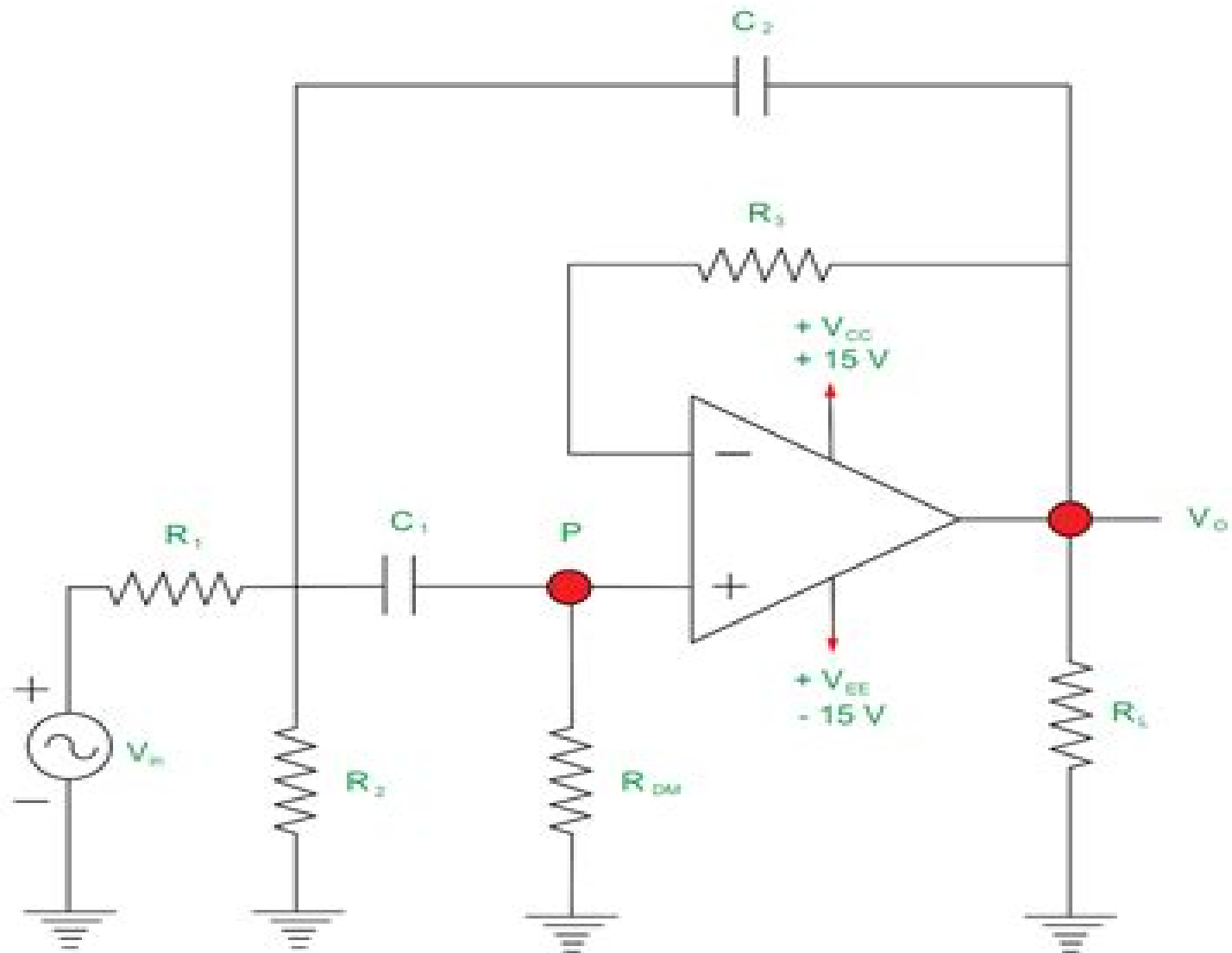
FIG : Multiple Feedback Narrow Band Pass Filter
