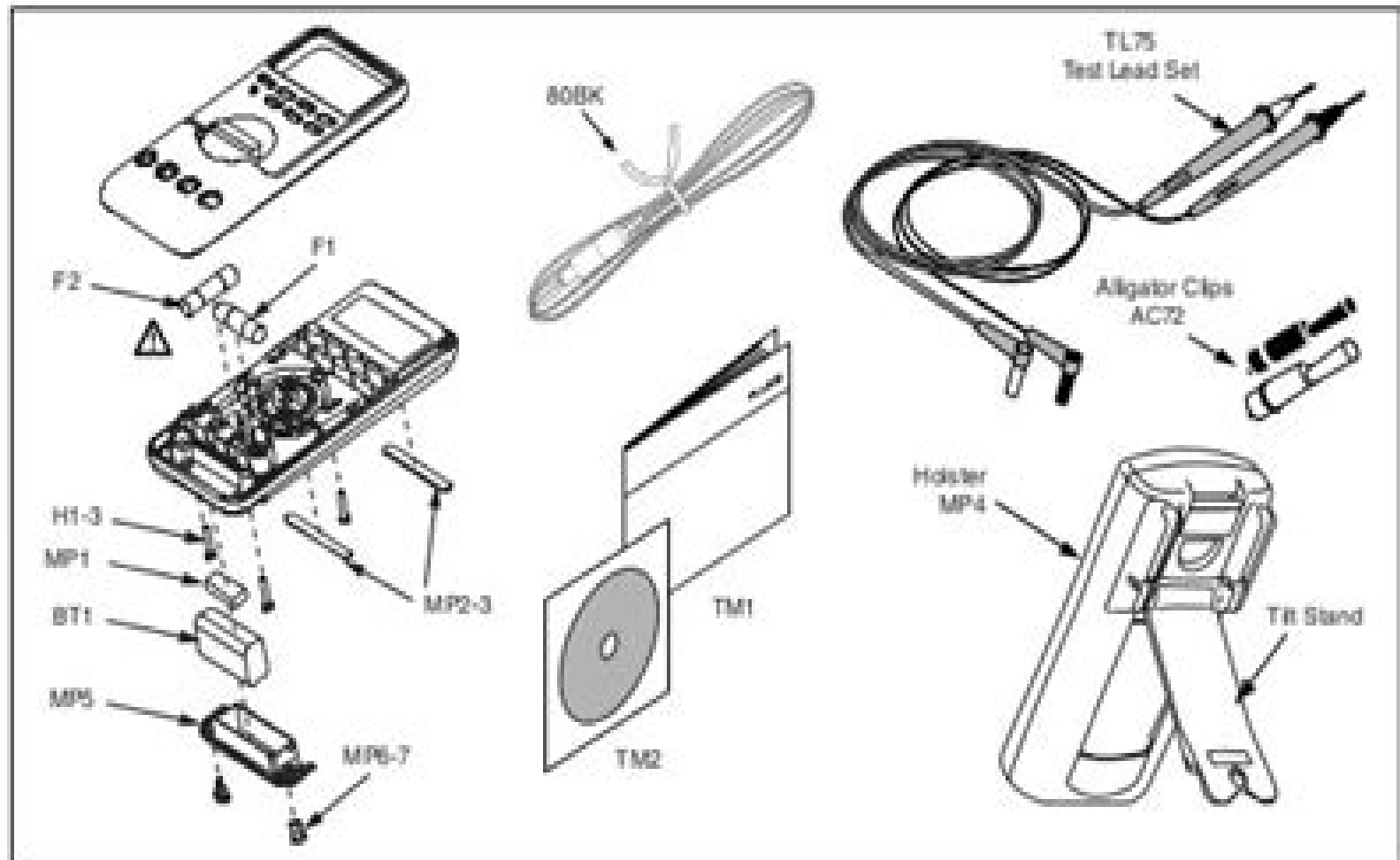
Figure 12. Replaceable Parts
