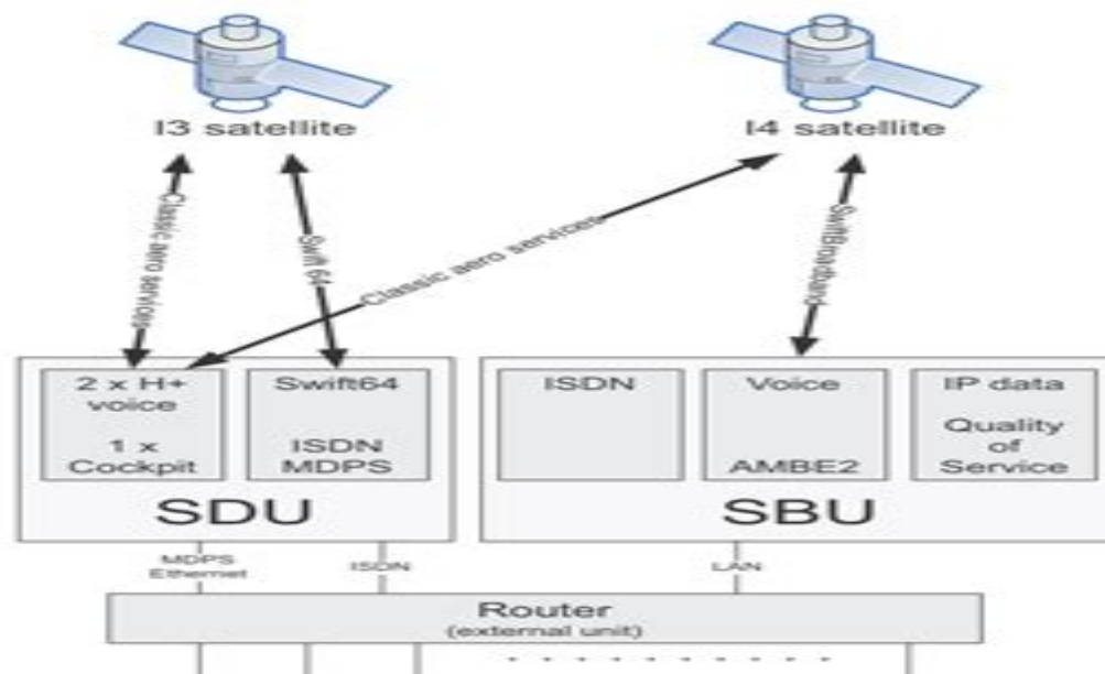
Figure 2-2: Satellite coverage of data and voice services
