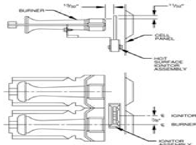
Fig. 9—Position of Ignitor to Burner
