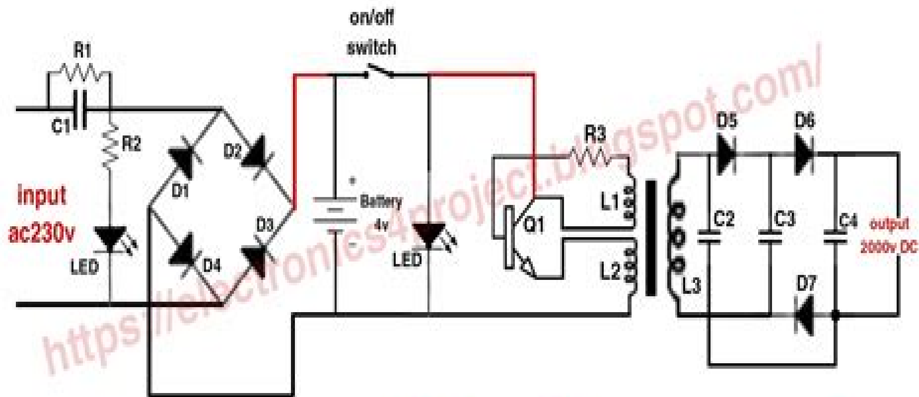
high voltage generator circuit diagram
