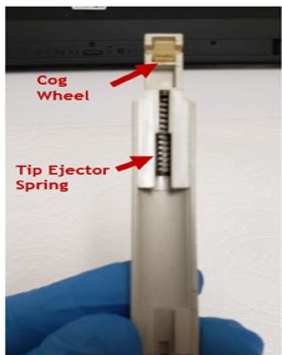
Tip Ejector Pusher Mechanism w/ Cog Wheel and Spring
