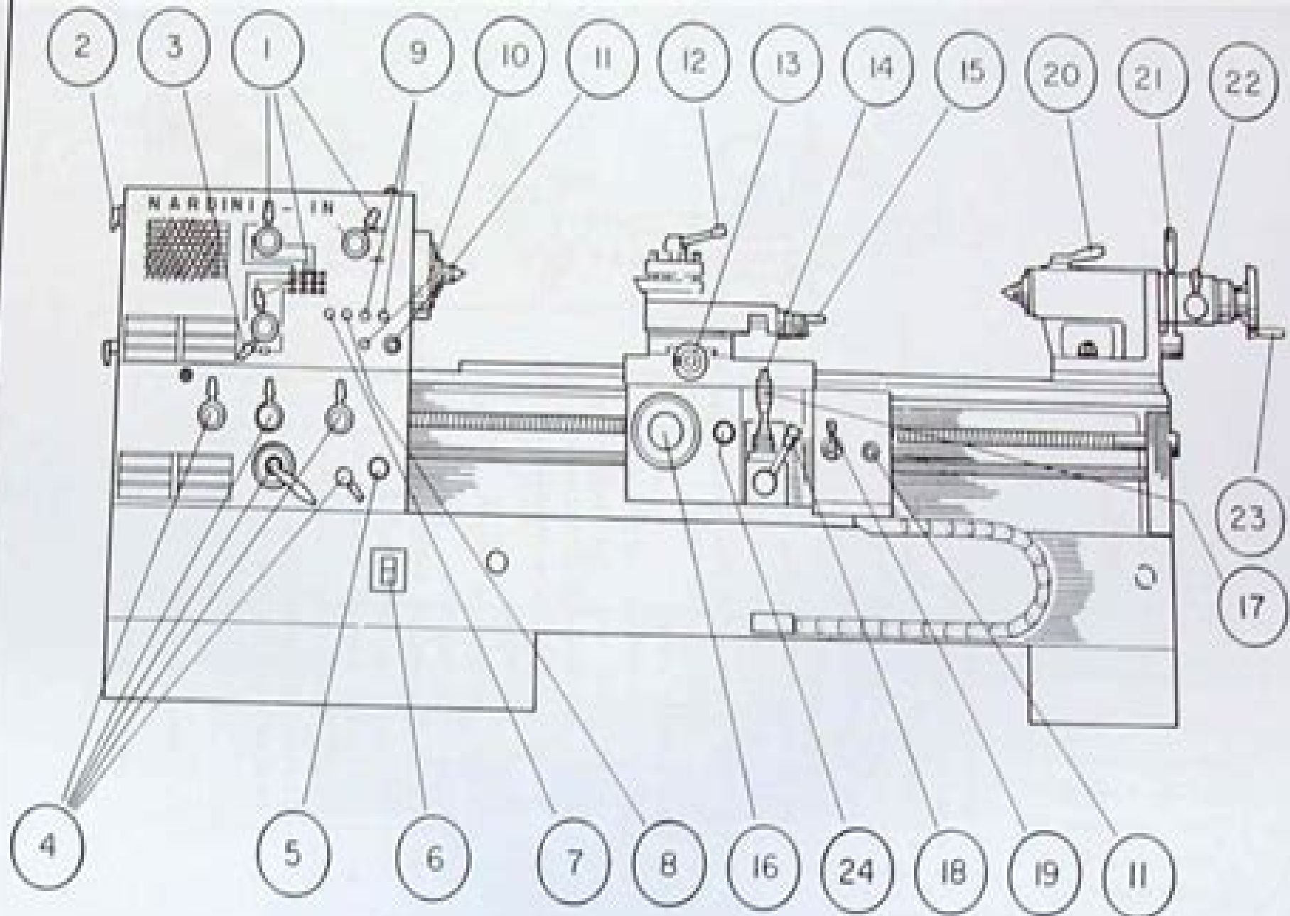
FIG. 5 LATHE CONTROLS
