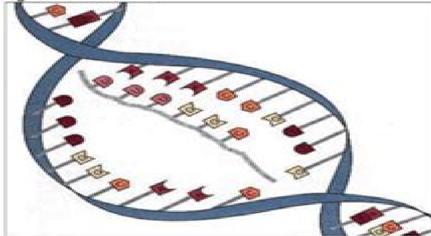
Figure 20.1 DNA Strand
