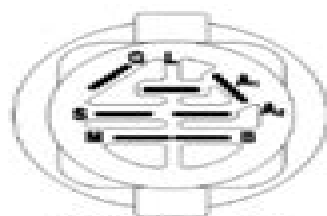
IGNITION SWITCH
