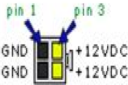
ATX 4 pin Molex 12V P4 Connector
