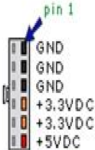
6 pin AUX Connector
