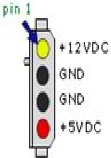
4 pin Molex peripheral Connector
