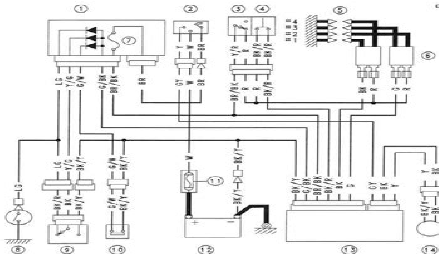
Ignition System Circuit
