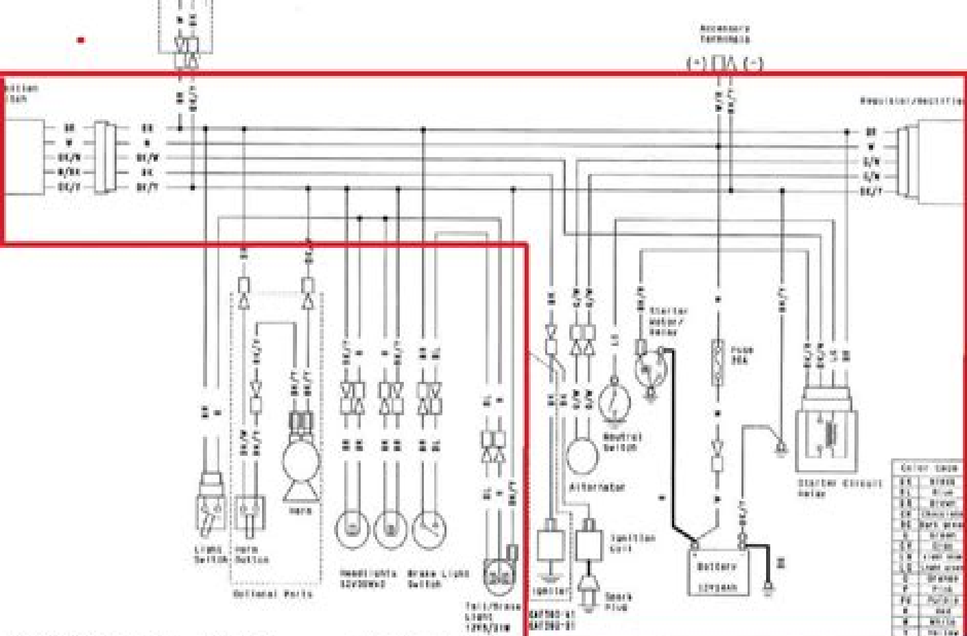
Ignition Switch Connections
