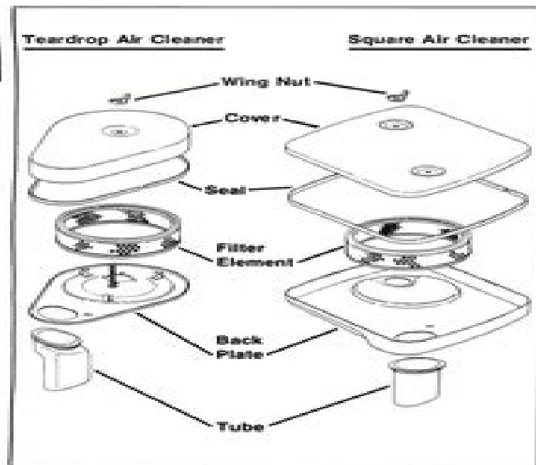
Figure 3-1. Air Cleaner Components
