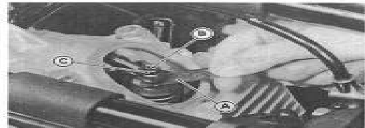
A. Thickness Gauge B. Adjusting Screw
