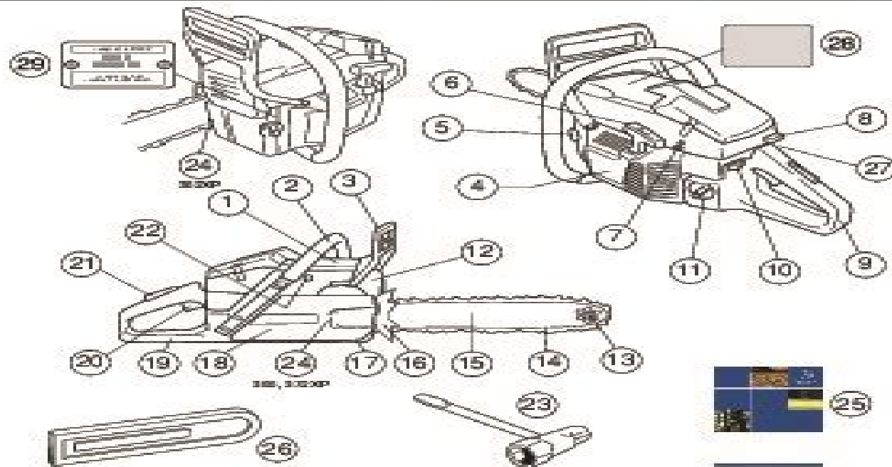
What is what on the chain saw?
