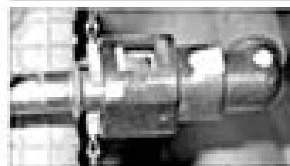
13 13a The fuel pump fitting, remove both ends with your fingers, then pull the fuel pipe and the fitting apart
