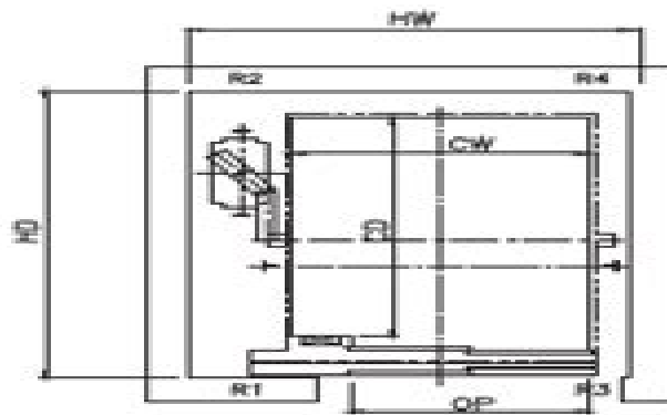
HOISTWAY PLAN (TYPICAL FL)
