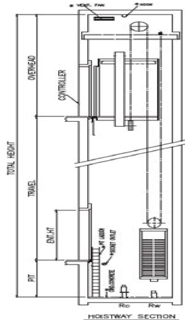
HOISTWAY SECTION
