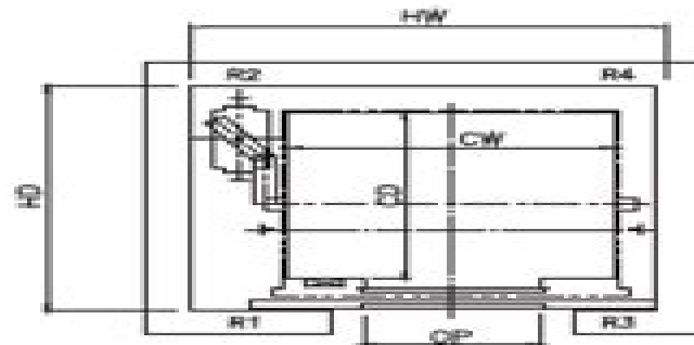
HOISTWAY PLAN (TYPICAL FL)
