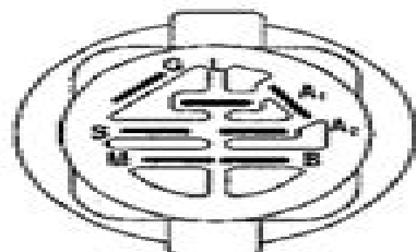
IGNITION SWITCH
