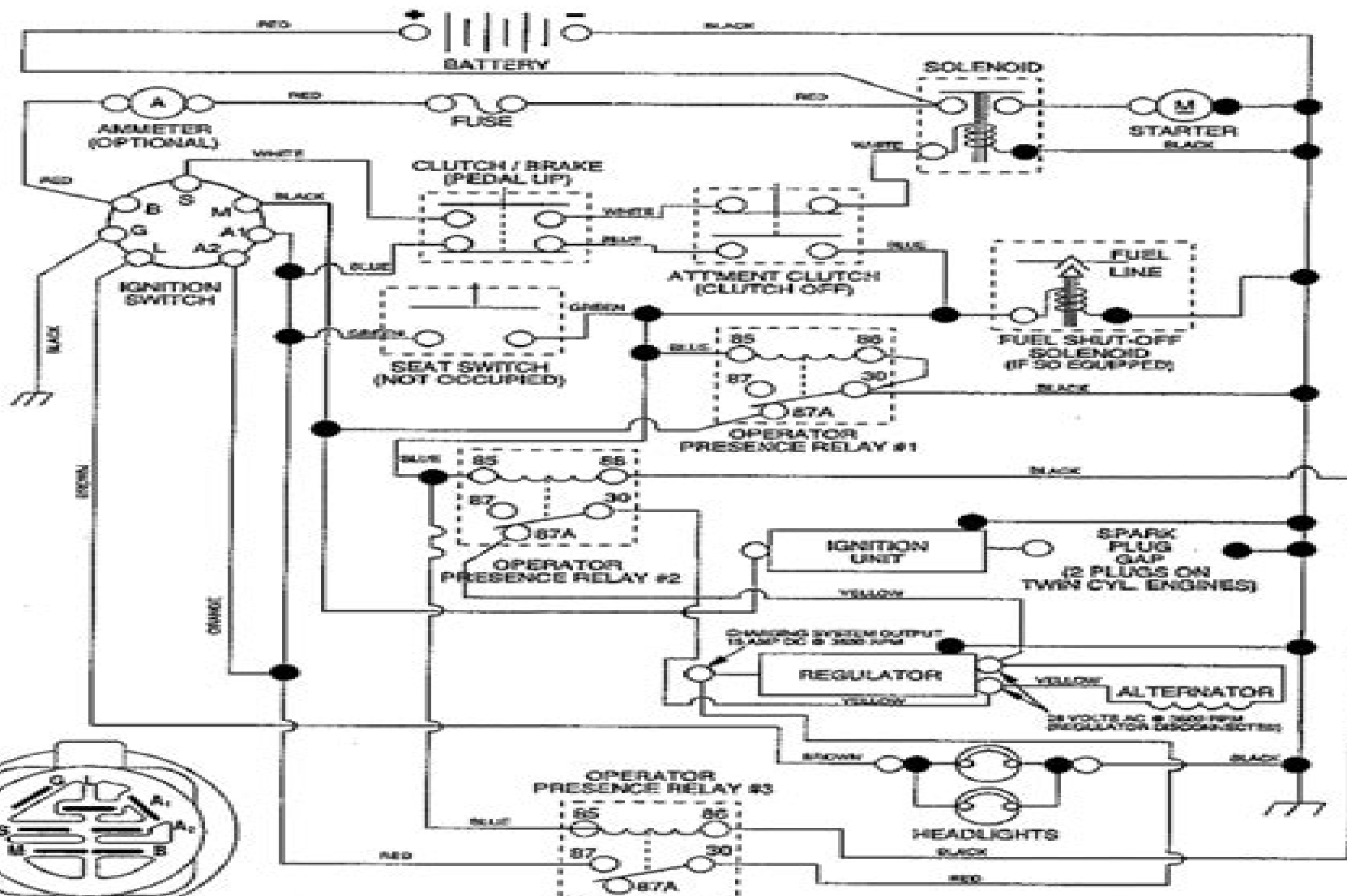
IGNITION SWITCH
