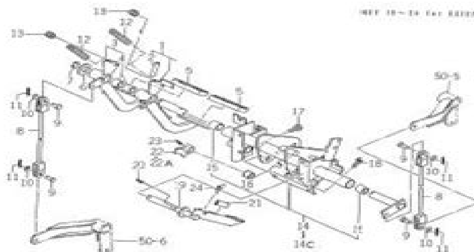
FIG. 52 BRAKE PEDAL SYSTEM
